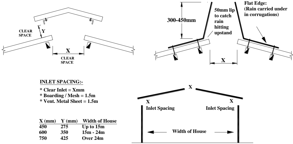
Figure 1 Ventilation details
