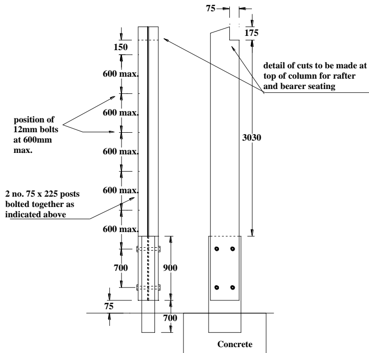
Figure 19 Internal column
