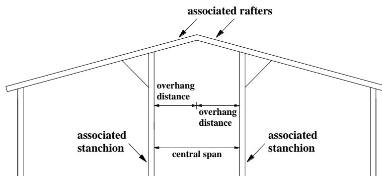
Figure 8 Double-sided house with central span
