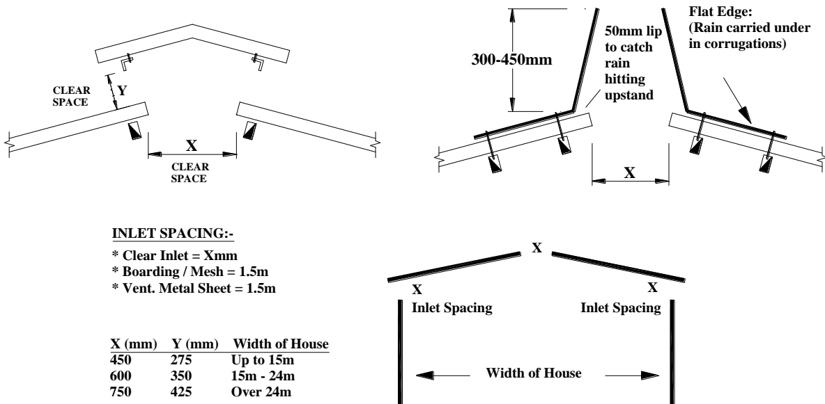
Figure 24 Ventilation details
