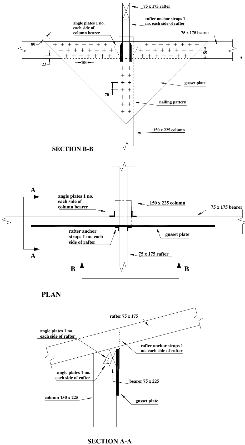
Figure 20 Top of internal column: connections
