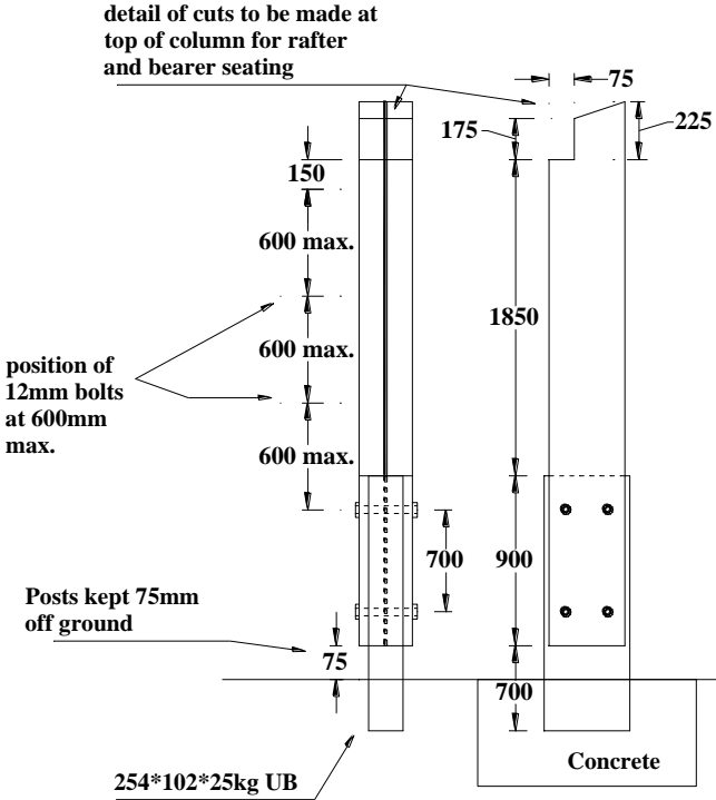
Figure 16 External column
