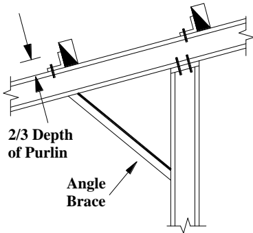
Figure 5 Bracing
