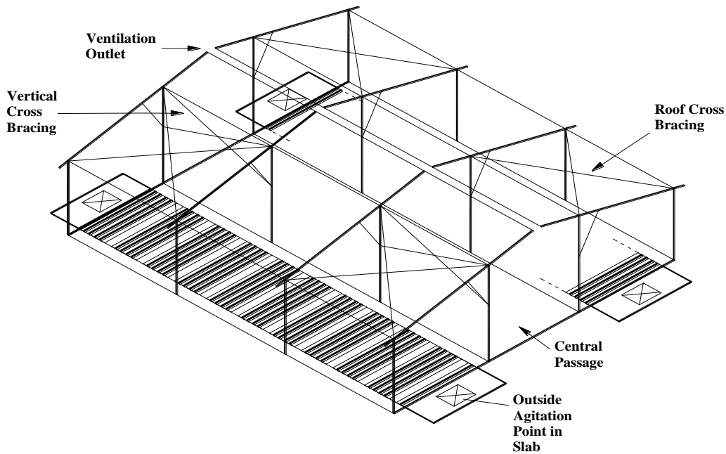
Figure 4 Double-sided simple steel frame house (3 bay/4.8m per bay/14.4m/tank-16.8m)
