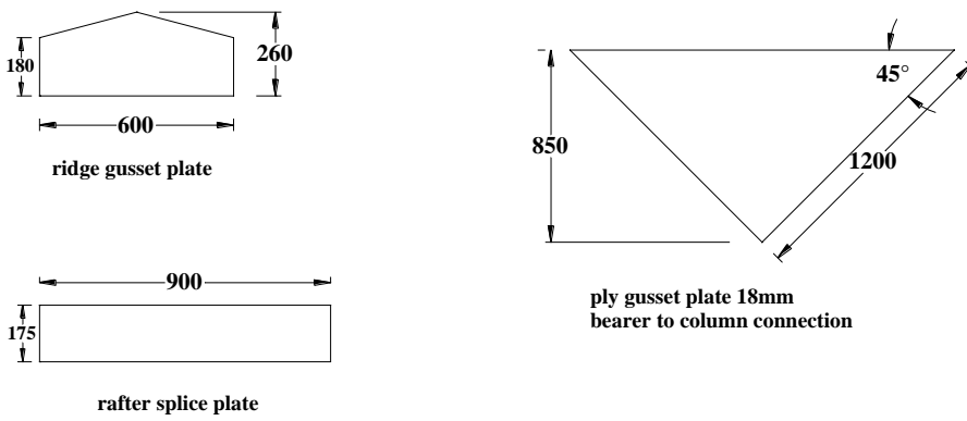
Figure 21 Gusset details
