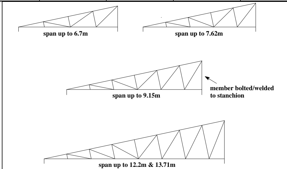
Figure 9 Triangulation detail for lean-to roof trusses
