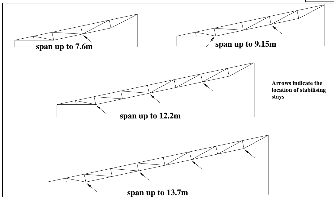
Figure 10 Bow truss details (truss depth = 500mm)
