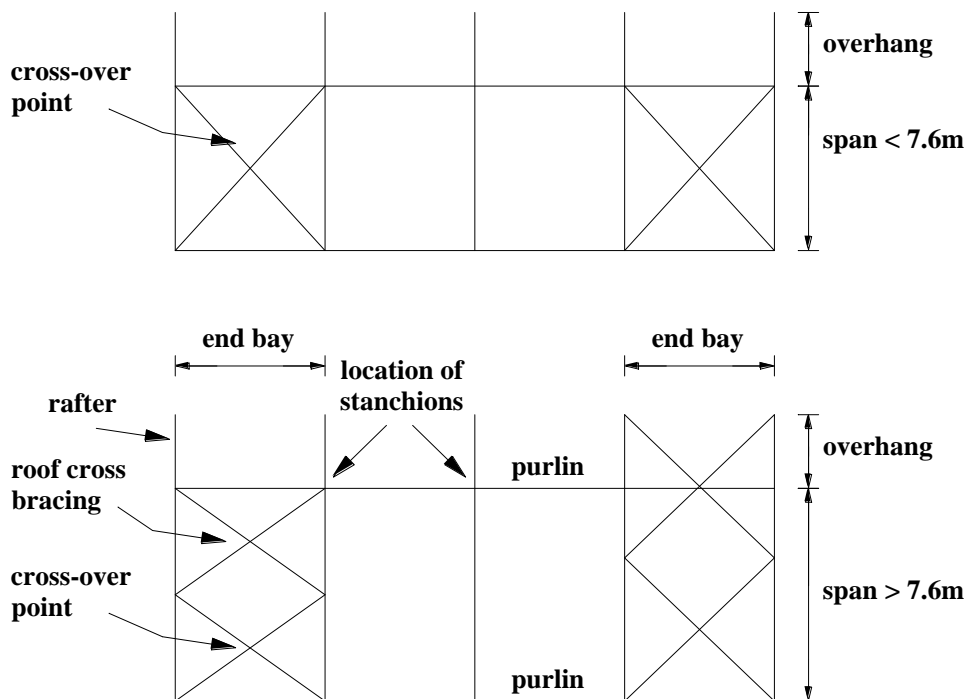
Figure 6 Plan view of single-sided house
