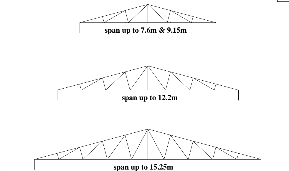
Figure 11 A-Roof trusses
