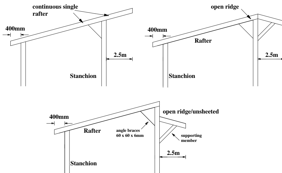
Figure 7 Interpretation of overhang options
