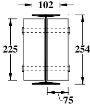
Figure 17 Column: Section
