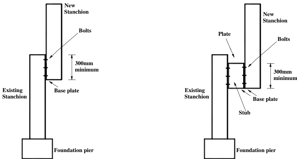
Figure 26 Grafting Detail
