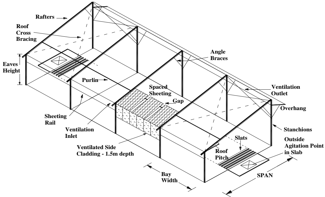
Figure 3 Single-sided simple steel frame house (4 bay)
