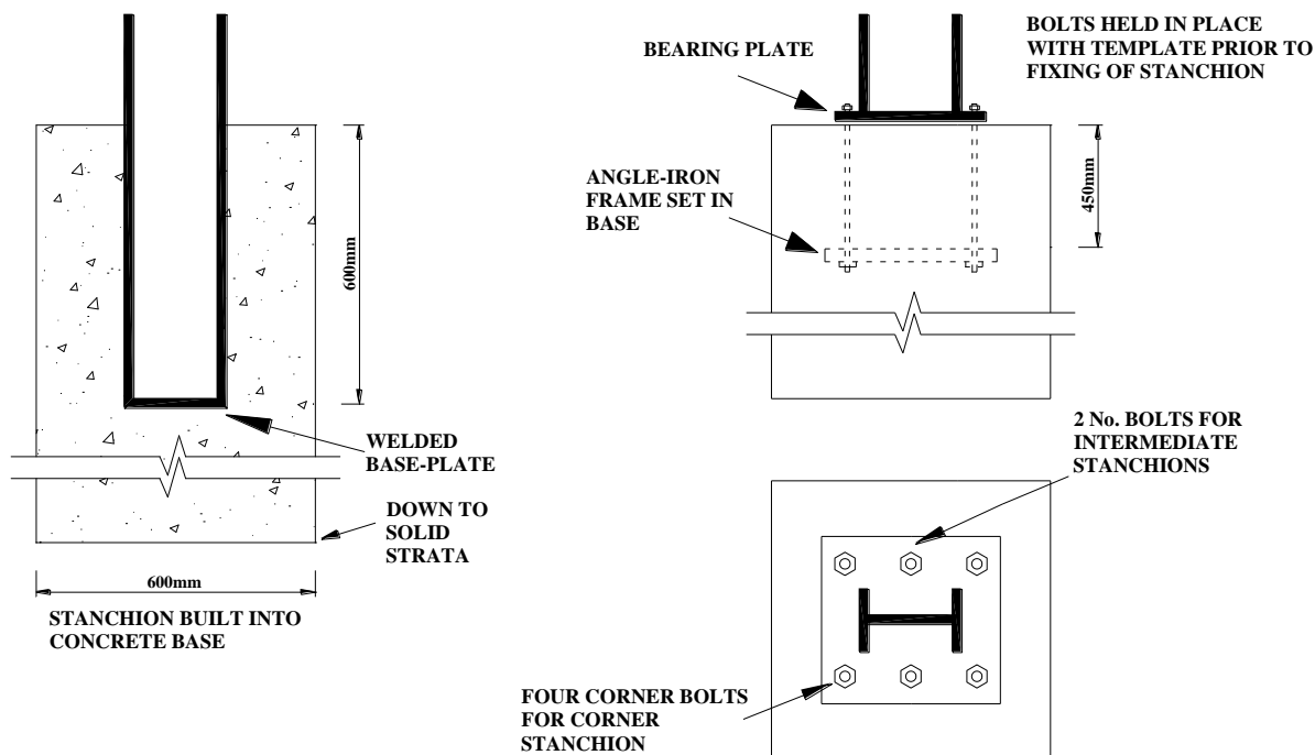
Figure 27 Stanchion base and pier details
