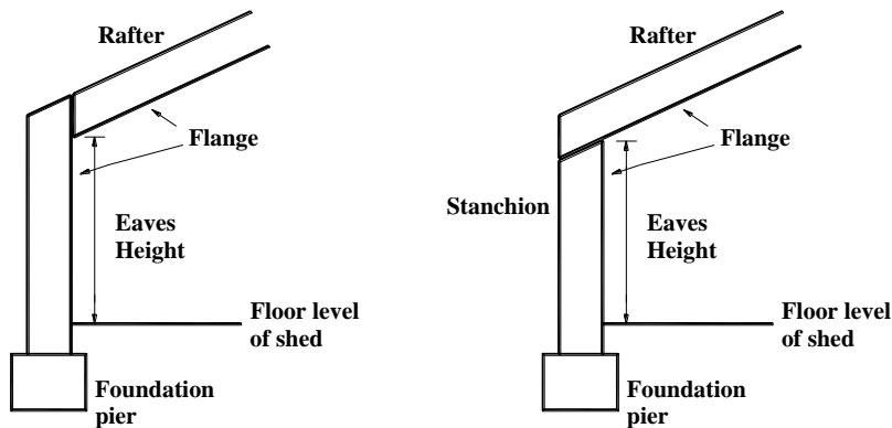
Figure 23 Interpretation of eaves height
