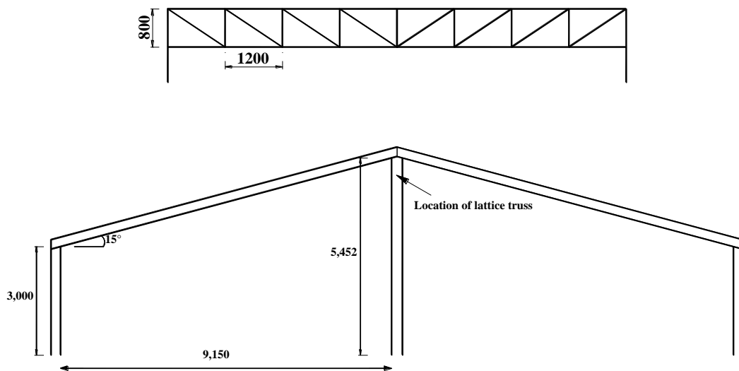
Figure 25 Lattice truss detail for back-to-back lean-to
