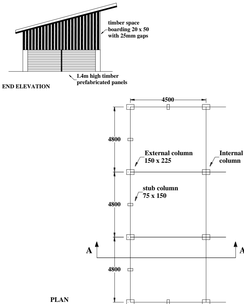
Figure 22 Plan and end elevation of timber building
