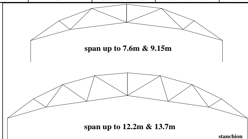
Figure 12 Triangulation detail for gathered (haybarn) roof truss
