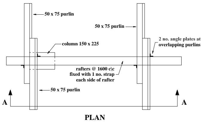
Figure 18 Top of external column / fixing of purlins
