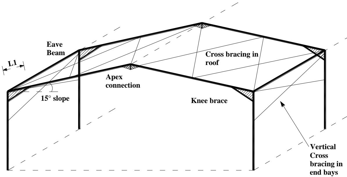
Figure 14 Elements in portal frame
