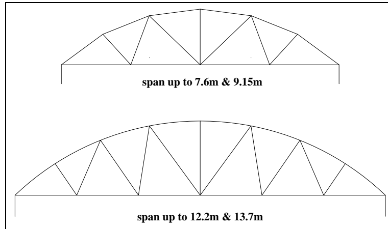
Figure 13 Triangulation detail for haybarn roof end truss
