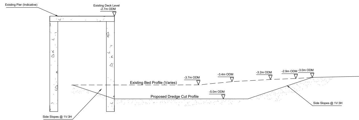
Cross Section A-A SCALE : 1:200
