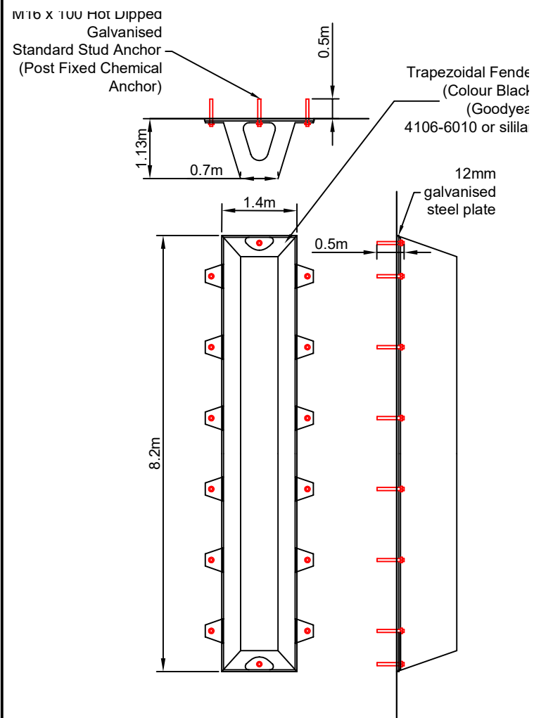
Rubber Fender Detail
