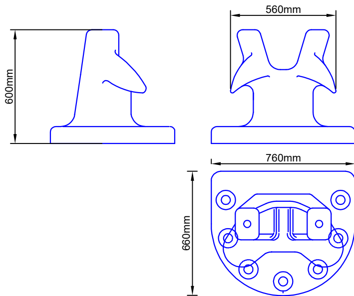
50 Tonne Twin Horn Bollard
