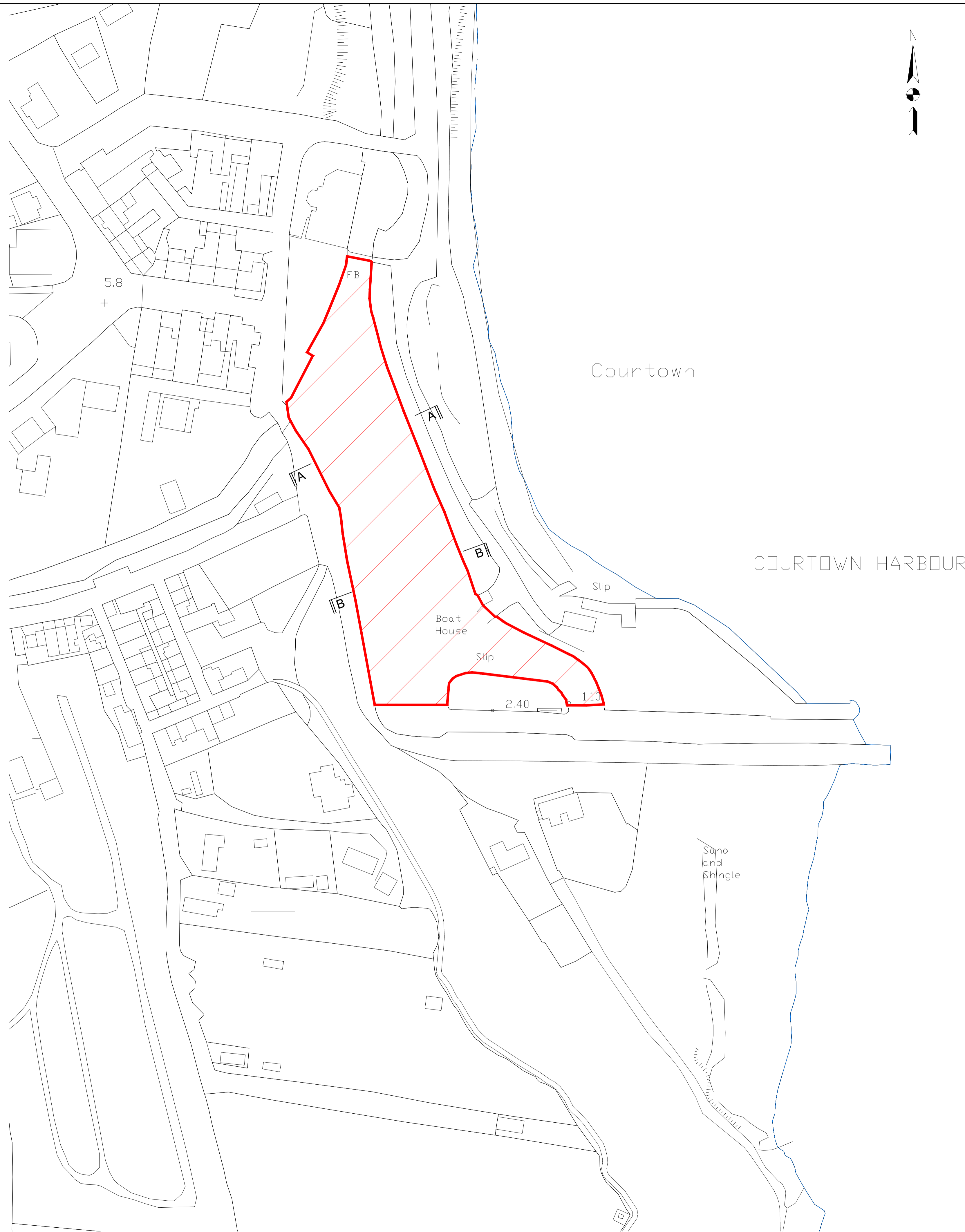
Layout Plan of Proposed Dredging Works Scale NTS
