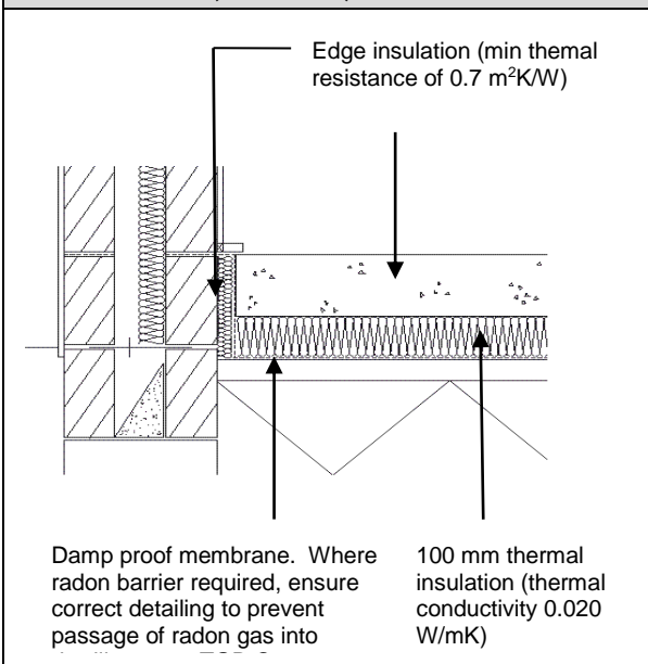
Diagram A4 Concrete slab-on-ground floor (Par. A3.1)
