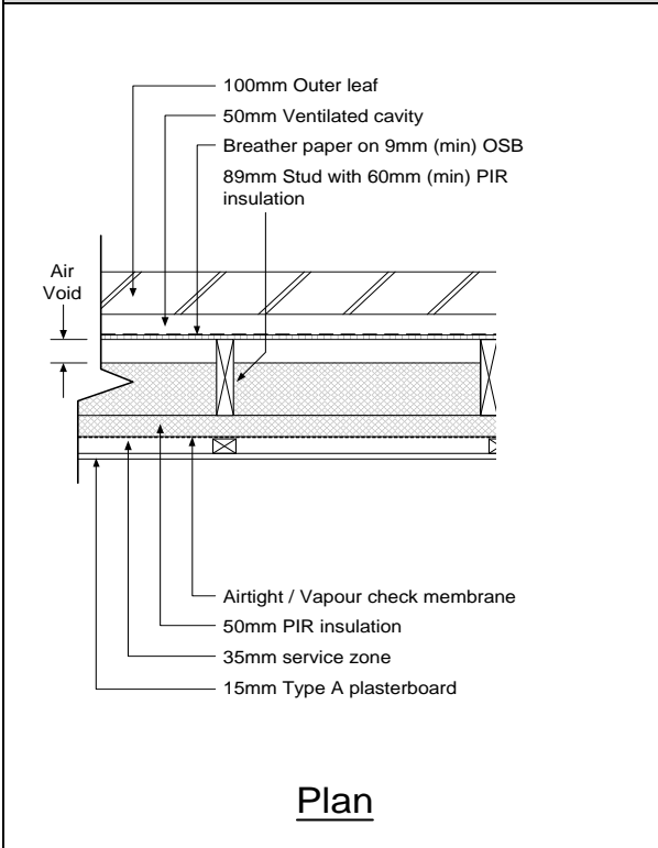
Diagram A2 Timber-frame wall (Par. A2.2)
