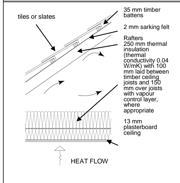
Diagram A3 Domestic pitched roof (Par. A2.2)
