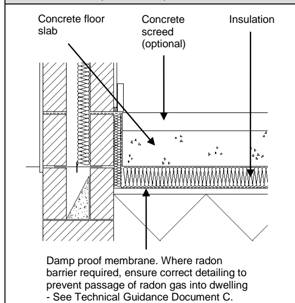
Diagram B12 Concrete slab-on-ground floor, insulation under slab (Par. B.7.1)
