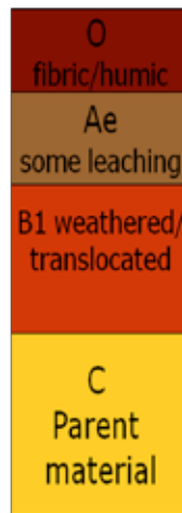
A brown podzolic profile with a topsoil comprising a thin, acid, peaty, upper layer overlying a yellow-brown lower topsoil layer, which in turn overlies a red-brown, iron-rich subsoil. Beneath the subsoil is the parent material from which the soil is derived.
