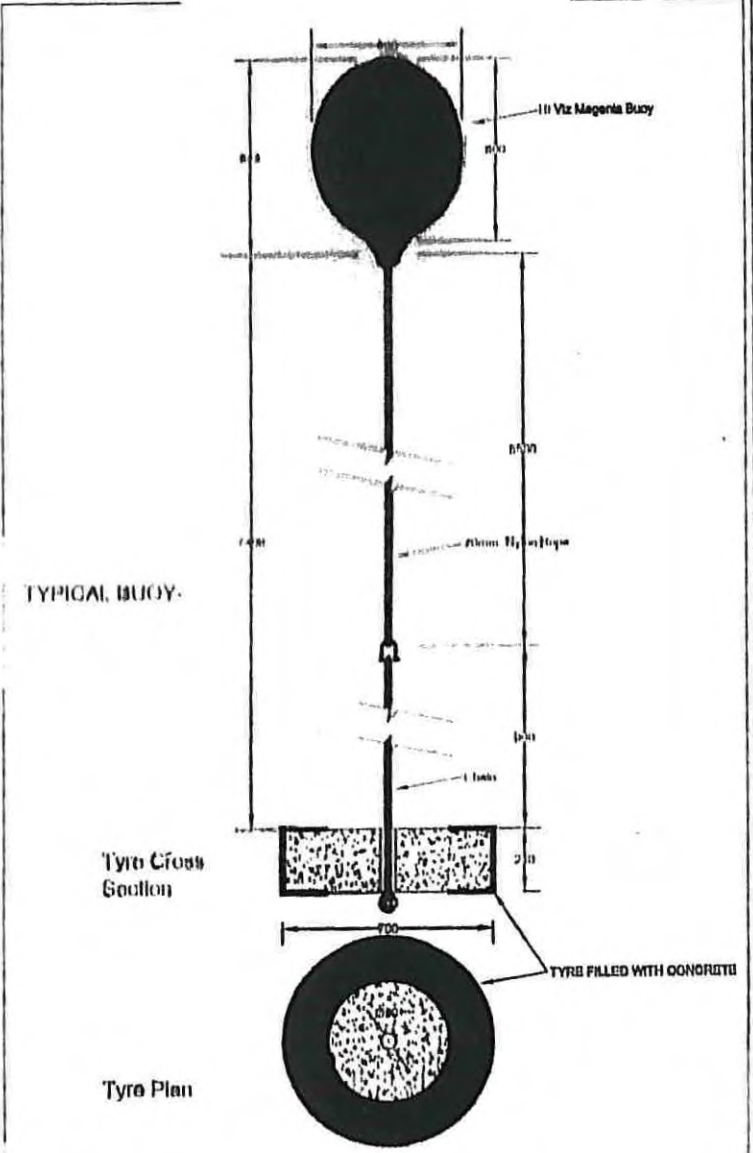
BUOY DETAIL 1:25
