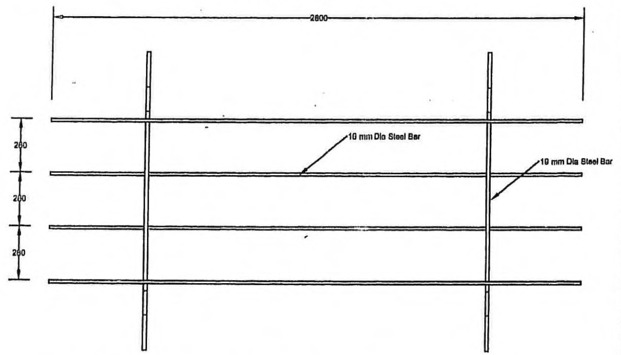
BAG & TRESTLE DETAIL 1:20
