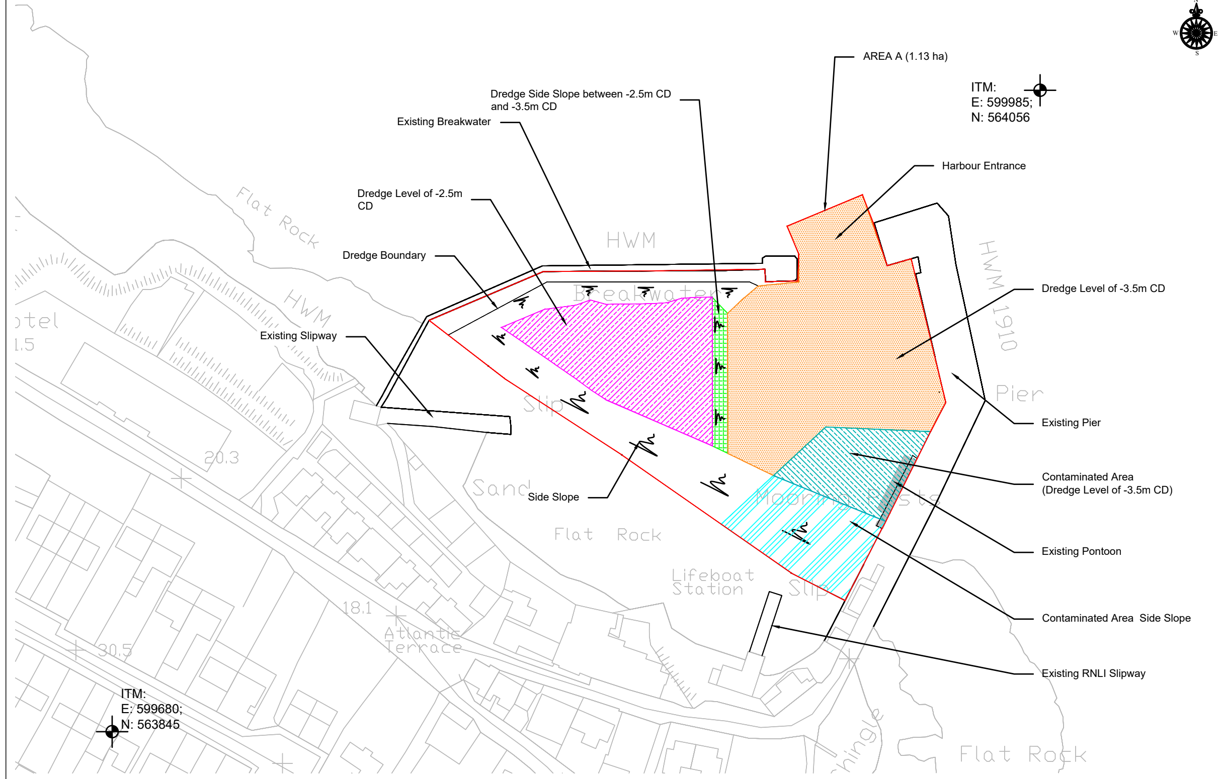
Ballycotton Harbour Plan Scale 1:1,250
